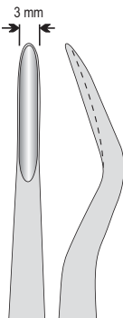
Fig. 2 MD-03-085 Bayonet Distal
